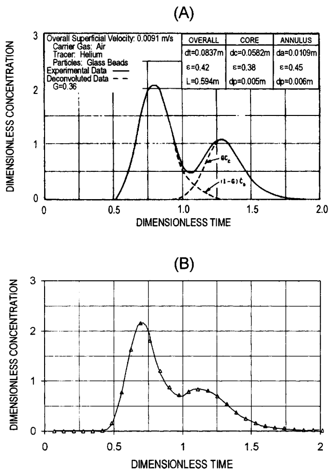
Figure 9. RTDs from heterogeneous bed with separation between zones.
