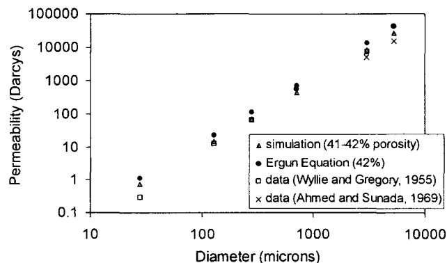
Figure 7. Prediction of permeability compared to Ergun equation and experiment.
