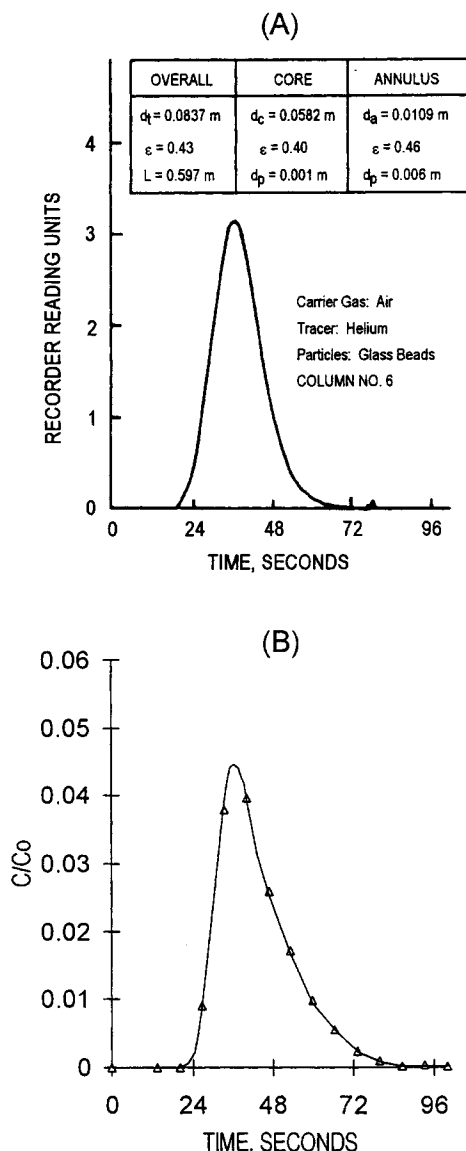
Figure 10. RTDs from heterogeneous bed with hydraulic communication between zones.
