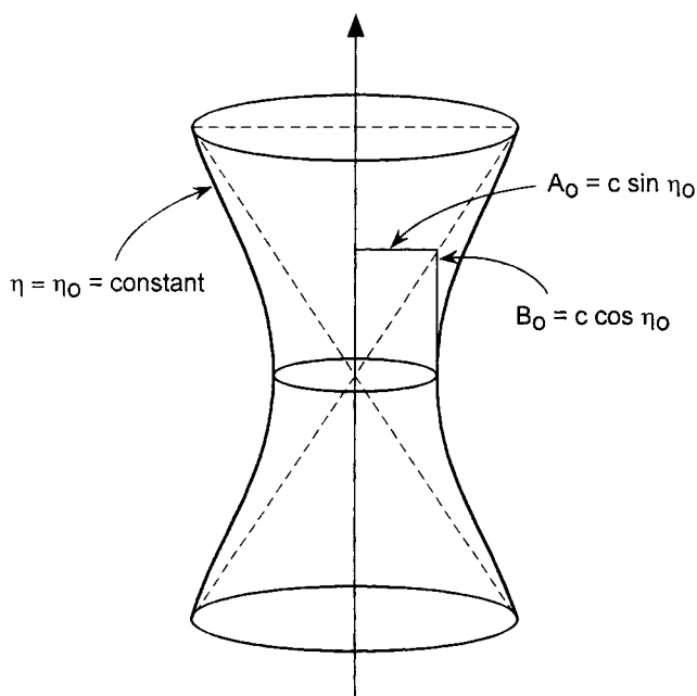
Figure 4. Hyperbolic Venturi.
